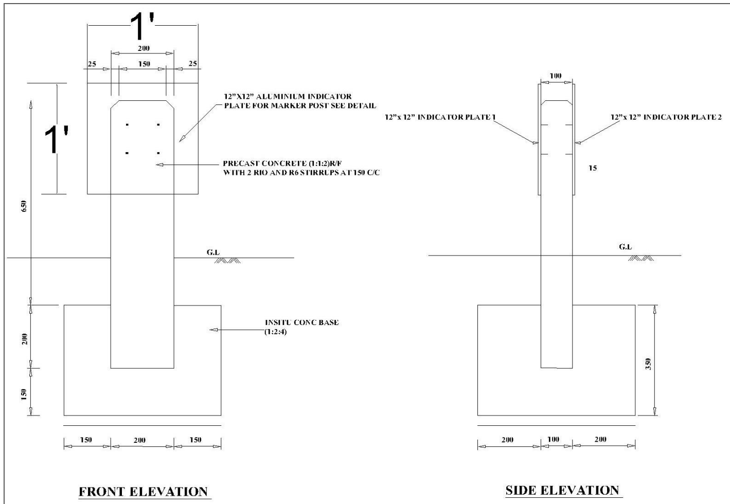
Indicator Plate 1
